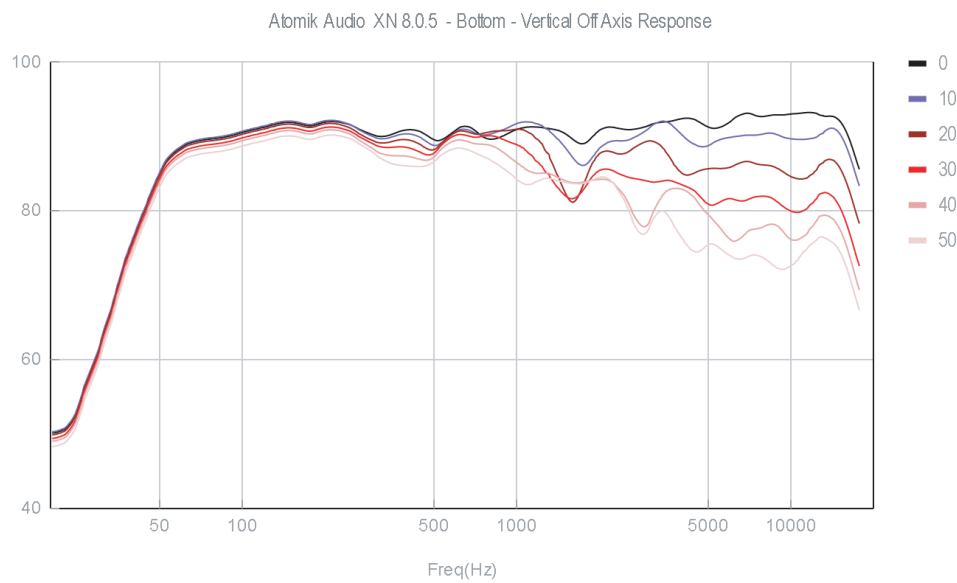
Bottom - Vertical Off Axis Response
